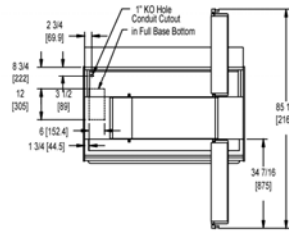
TOP VIEW (DRTSWG-3, 4 & 5)
