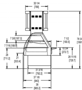
END VIEW (DRTSWG-3, 4 & 5)
